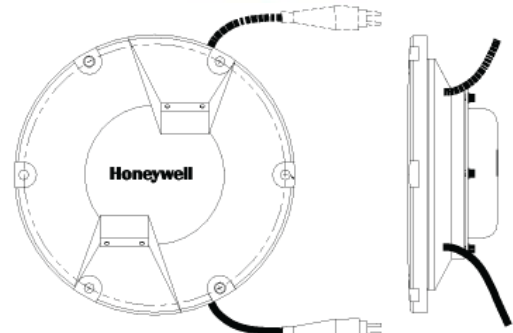
OUTLINE DRAWING
