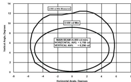
L-850A Isocandela Performance 2,500 CD White
