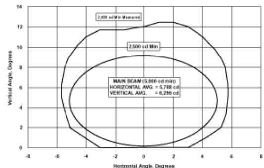
L-850F Isocandela Performance 2,500 CD White
