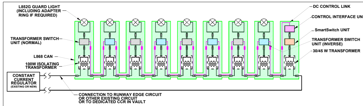
NON-MONITORED L852G GUARD LIGHT SYSTEM GENERAL ARRANGEMENT
