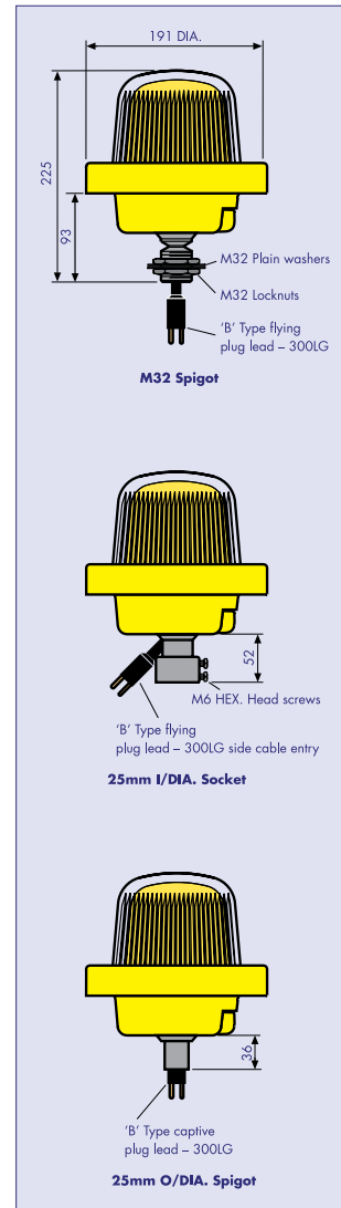
ZA163 general arrangement
